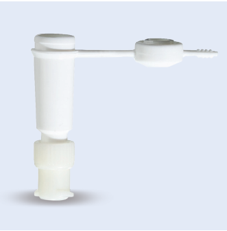
Freka Universal Funnel Adaptor For compatibility of: - ENLock Sets to ENFit Feeding Tubes - ENLock syringes to ENFit Feeding Tubes - for decompression with drainage bags
